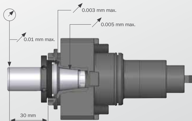
With QuickFlex® mill arbor adapter
