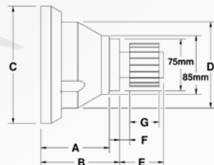
Standard Sleeve
