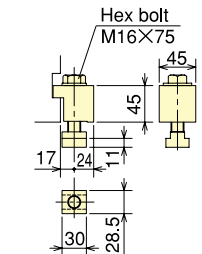
Clamping Device
