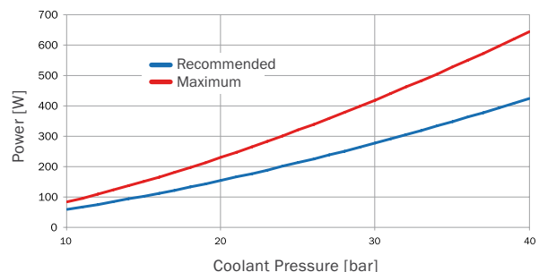
Power/Coolant Pressure
